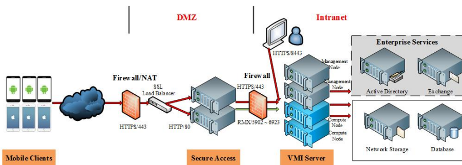
FIGURE 1-3. Trend Micro Virtual Mobile Infrastructure High Availability architecture
