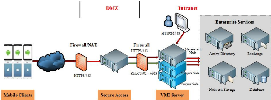
FIGURE 1-2. Trend Micro Virtual Mobile Infrastructure Multiple Server Installation Model
